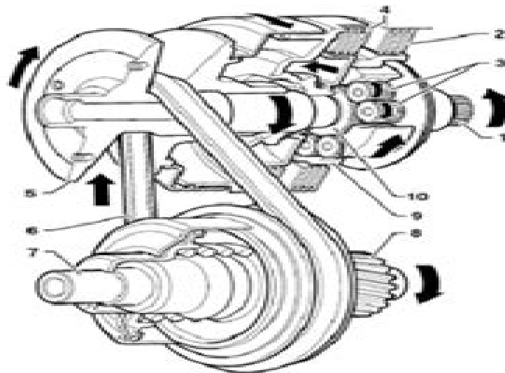
Fig. 21: Pulleys & gear train
