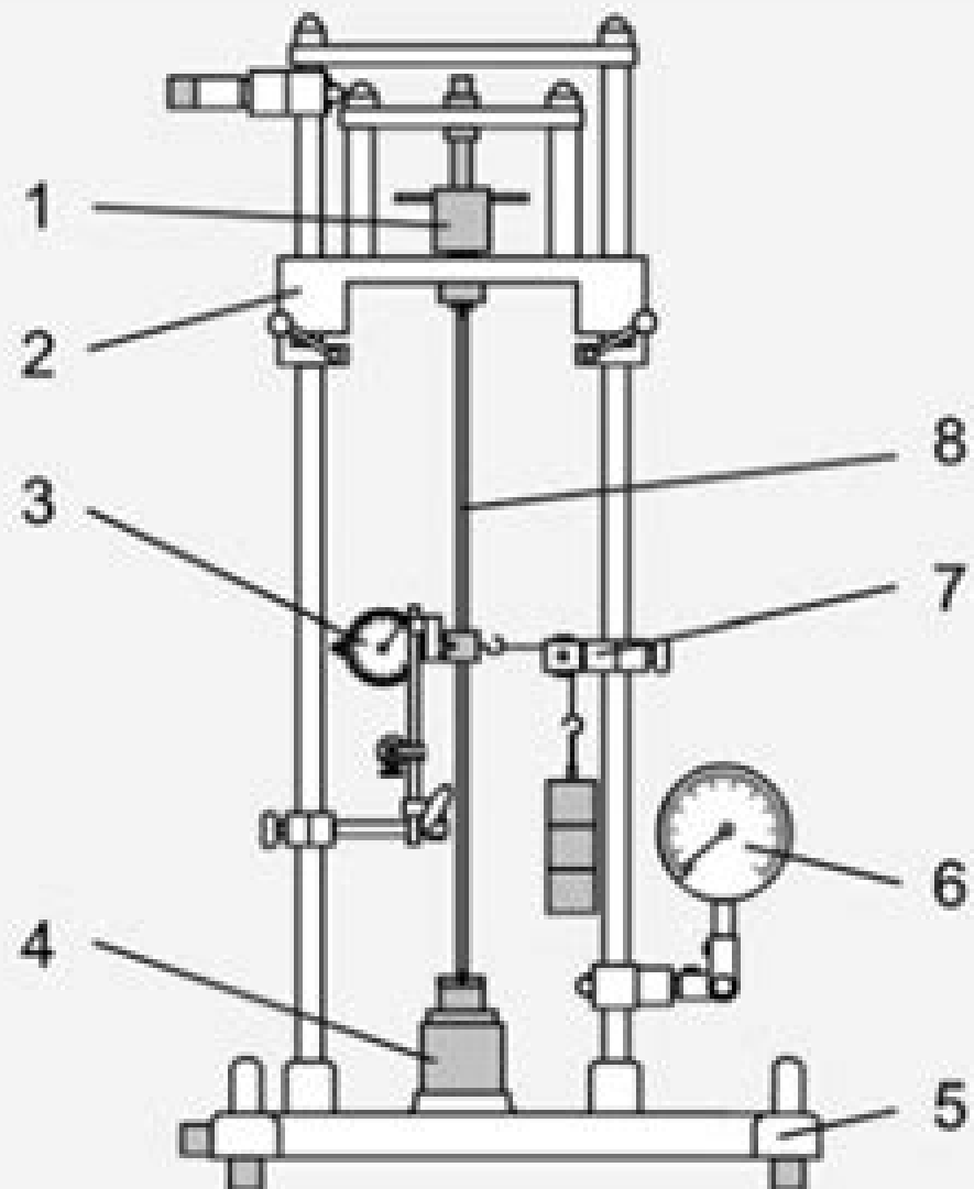
1 spindle, 2 height-adjustable load-carrying cross-arm, 3 dial gauge for lateral deflection of test bar, 4 load cell, 5 frame, 6 pressure gauge, 7 device to generate a transverse load, 8 test bar
