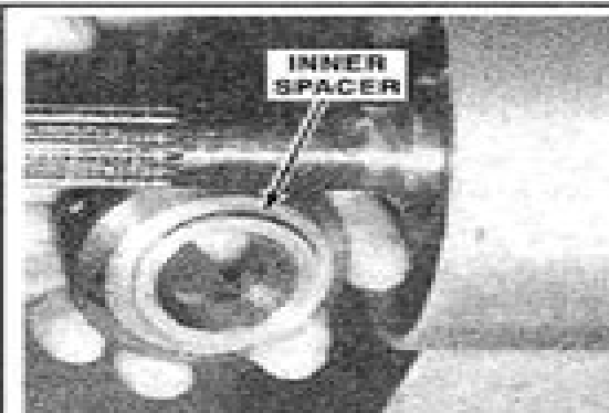
Fig. 78 For installation position the inner spacer first...
