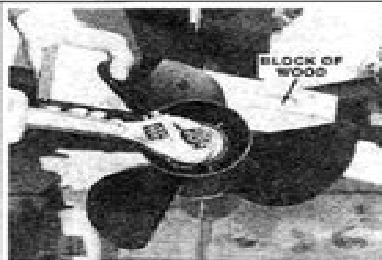
Fig. 74 To remove the nut use a block of wood to keep the prop from turning
