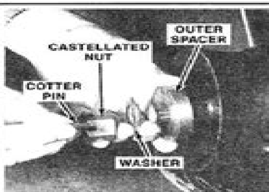
Fig. 80 Then install the outer spacer, washer (if used), nut and cotter pin
