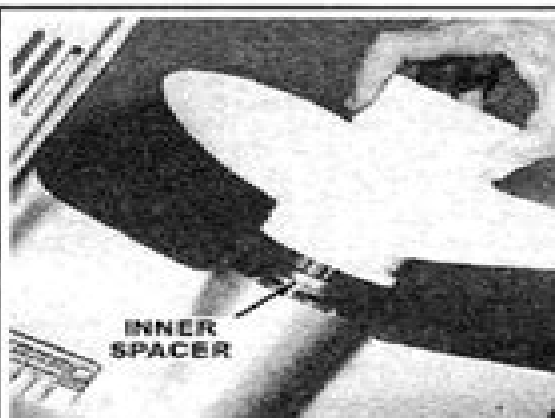
Fig. 79 ... with the shoulder facing the prop
