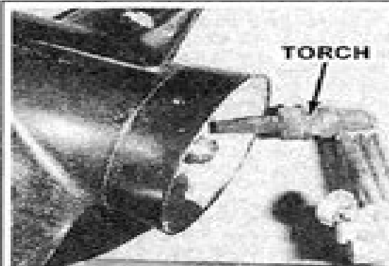
Fig. 75 A stuck propeller can be freed with heat...
