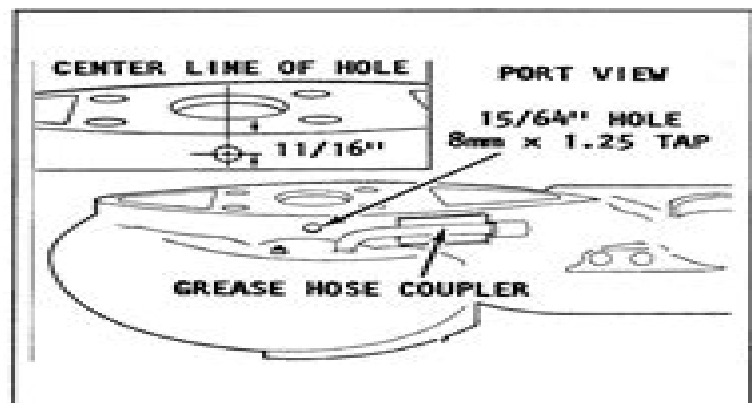
Fig. 40 On models not equipped with a flushing plug, a hole should be drilled and tapped to receive a plug as illustrated.
