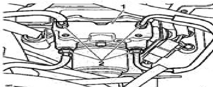
1. ABS modulator 2. Brake line unions
