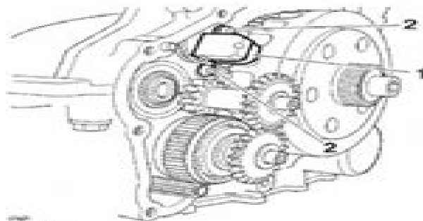
1. Sensor 2. Fixings
