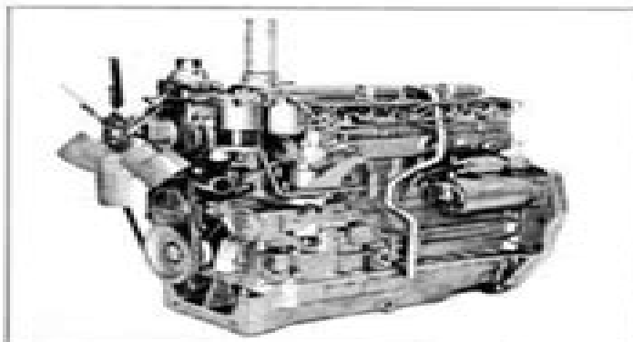
Fig. 1 - Front Left-Hand View of A6.354 Engine (Early Engine with Series Type Fuel Filters Shown)
