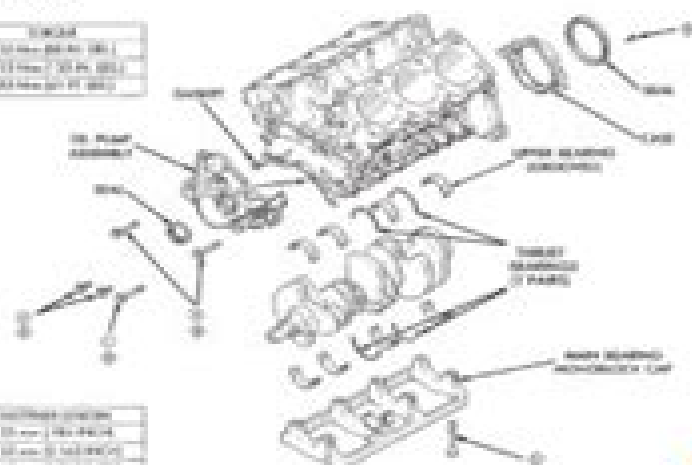
Fig. 37 Crankshaft and Cylinder Block
