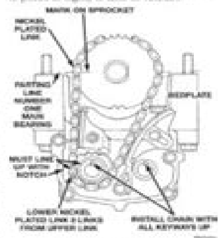
Fig. 42 Balance Shaft Timing
