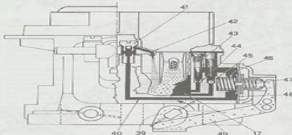
Fig. 7.7 Carburettor acceleration phase (Sec 3)
