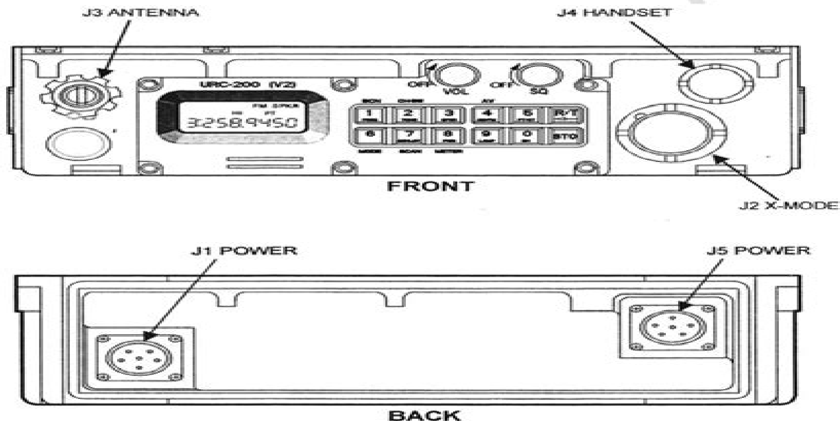
Figure 3-2. URC-200 (V2) Interfaces
