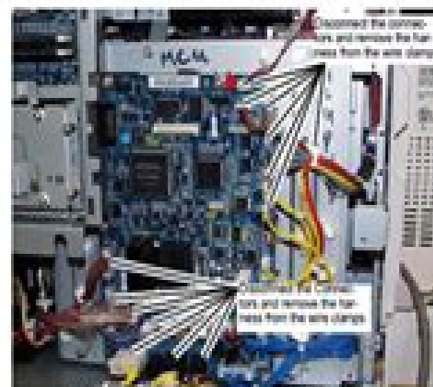
Figure 2 Disconnecting 13 of the connectors on the MCU PWB
