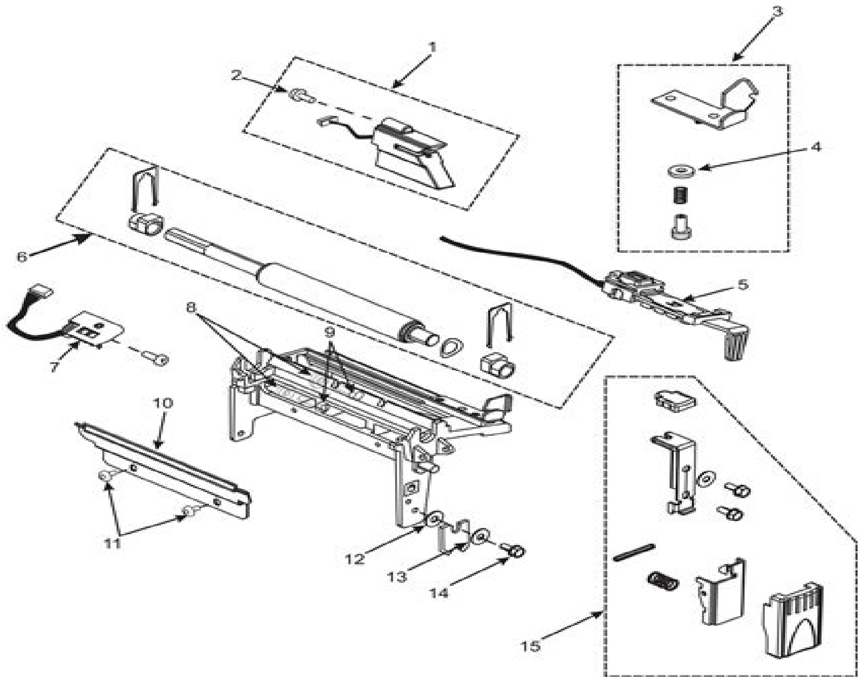
Figure 5-4. Platen Assembly
