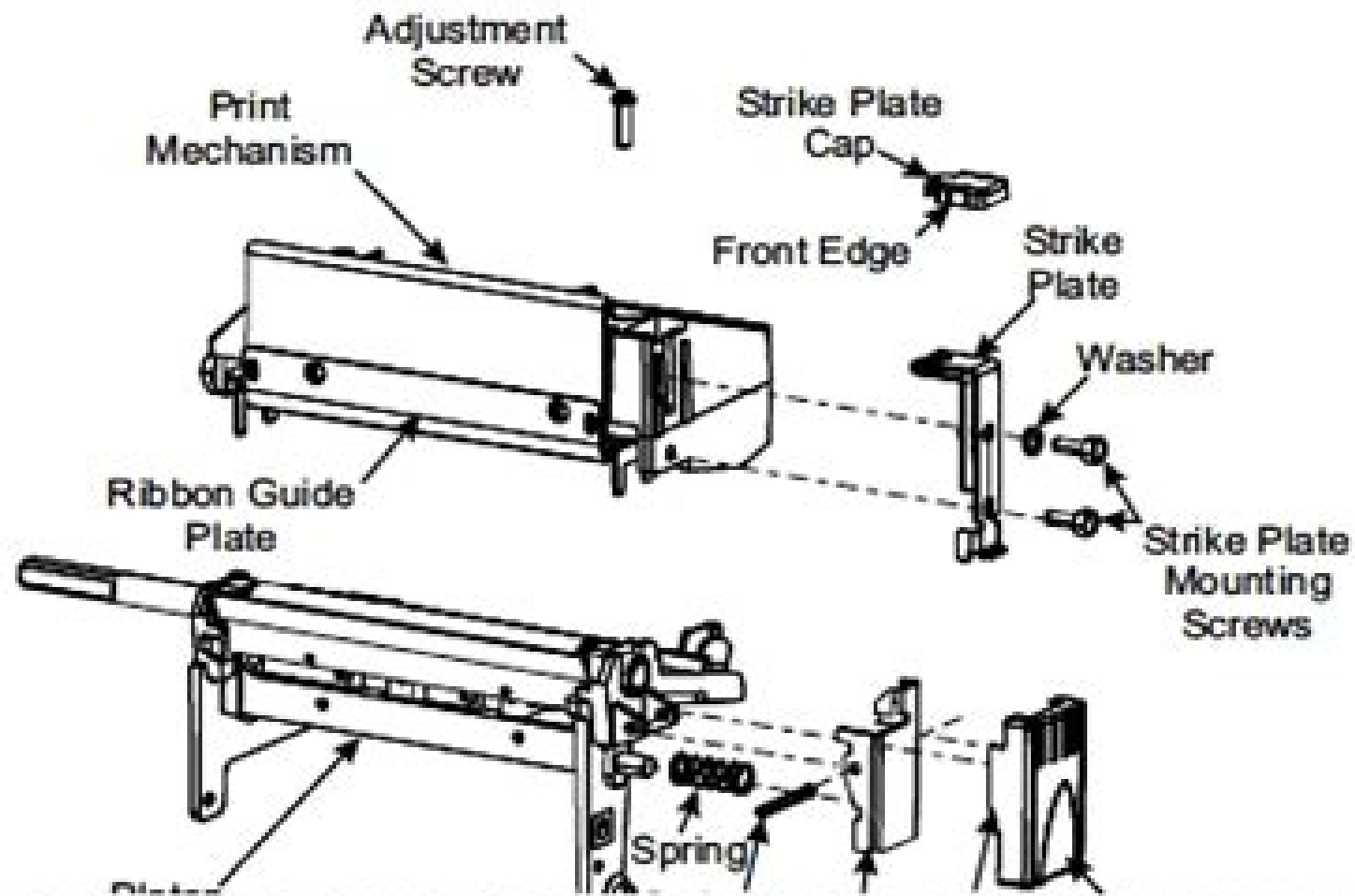
Figure 4-11. Latch Kit Parts
