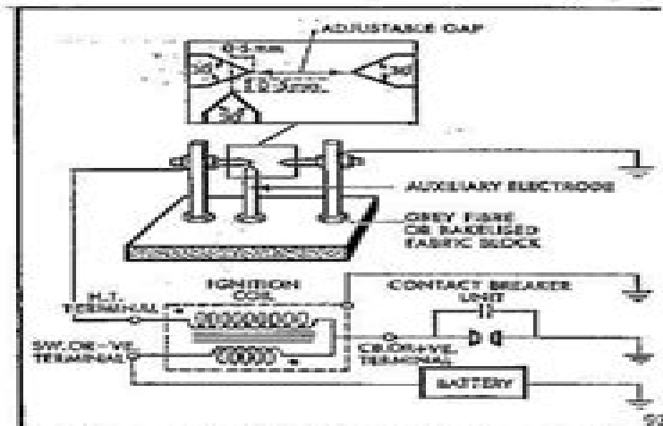
Fig. H3. Ignition coil test rig
