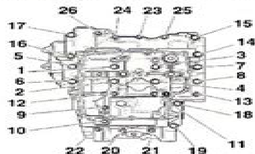
Crankcase Fixing Tightening Sequence
