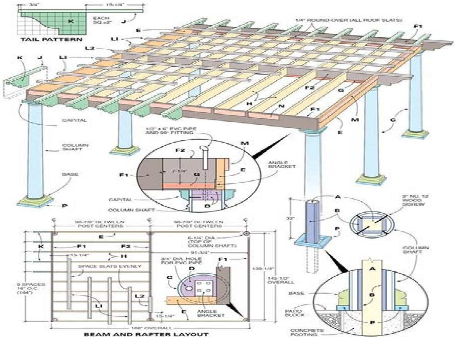
Figure A: Pergola Details
