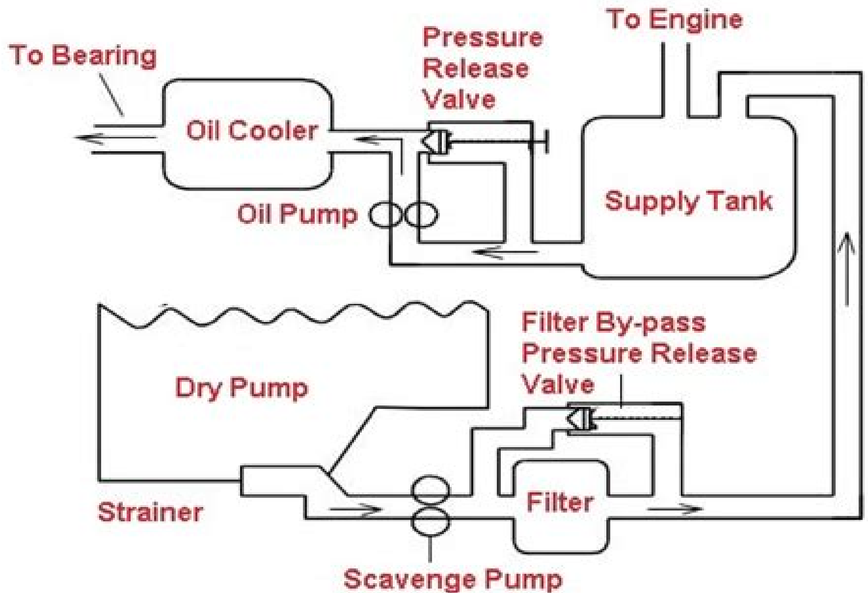
Dry Sump Lubrication System
