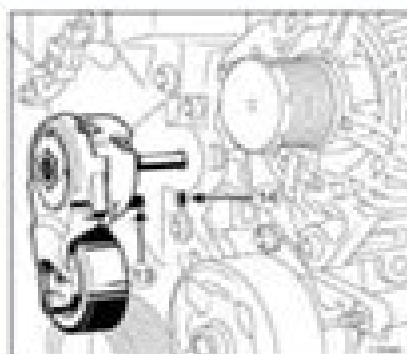
2 Refit the new auto tensioner by inserting leg (15) into its housing (14).
