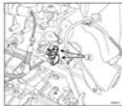
2 Loosen the heater matrix cooling hoses at (2).
