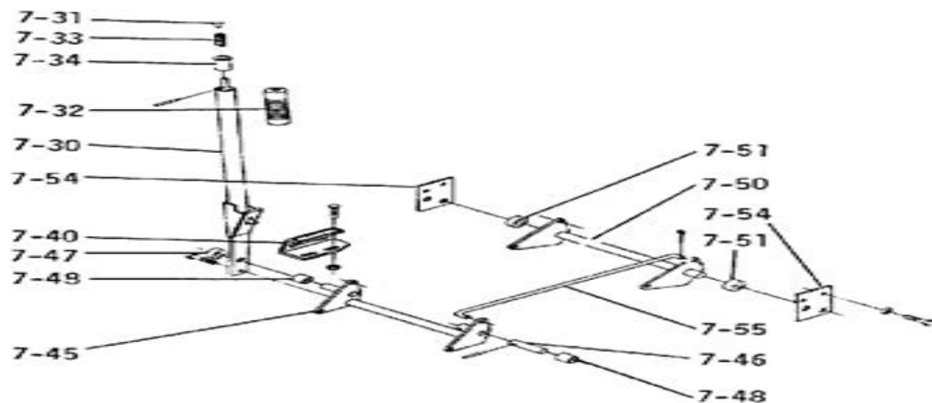
TYPICAL MANUAL LIFT LINKAGE — 1LR MODELS
