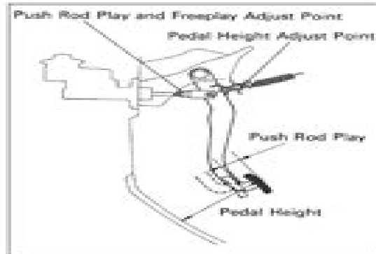
14.5a The clutch pedal pushrod play, pedal height and free play adjustments are made by slackening the locknut and turning the threaded adjuster
