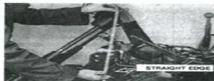
Fig. 156—With hitch at maximum height, distance between center of lift link pin and top face of rear frame should be 15.93 inches (404 mm).
