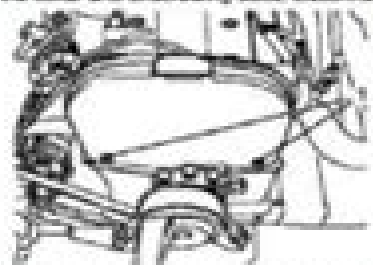
Fig. 2.89. Bolts for fastening the top of the belt toothed belt: 1 - bolts fastening
