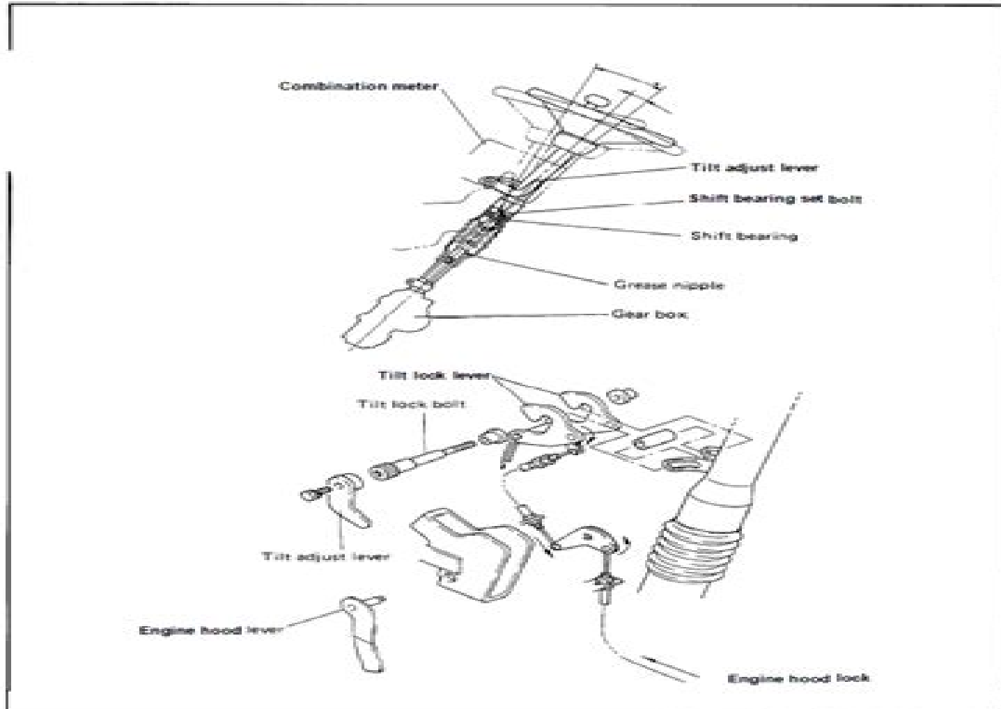
Steering Tilt System (1986.8~1989.8)
