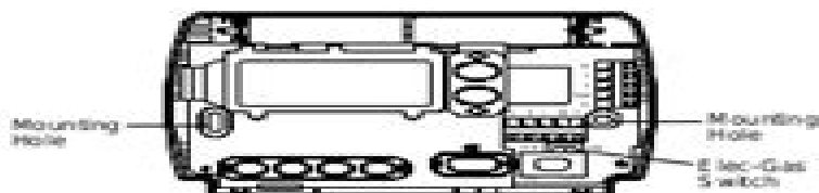
Figure 1 – Thermostat base
