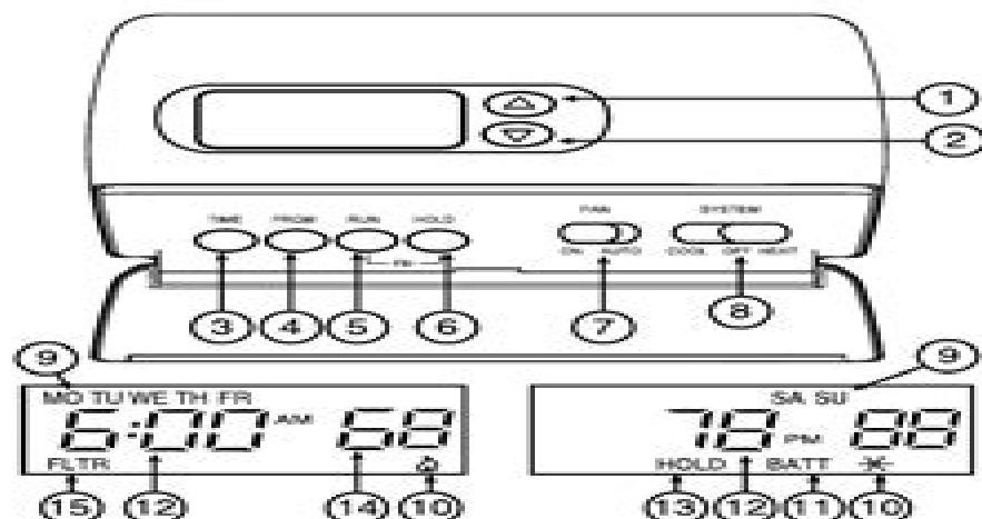
Figure 8. Thermostat display, buttons, and switches
