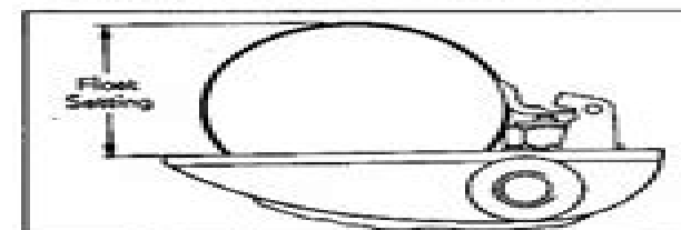
Fig. 15 FLOAT SETTING
