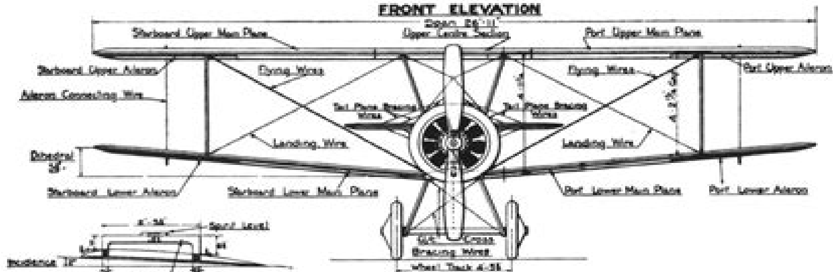
FIG. 3. FRONT ELEVATION
