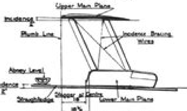
FIG. 4. POSITION OF UPPER MAIN PLANE WITH RELATION TO LOWER MAIN PLANE.
