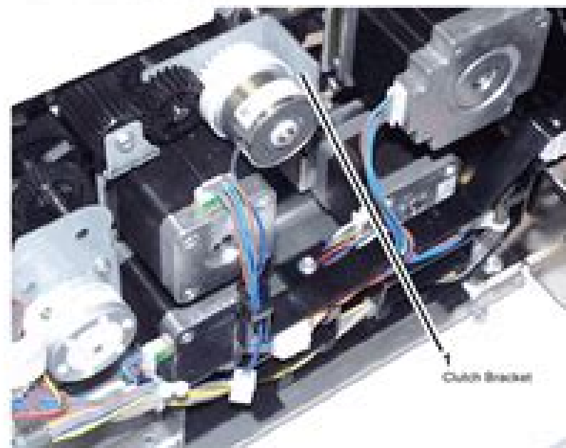
Figure 1 Clutch Bracket
