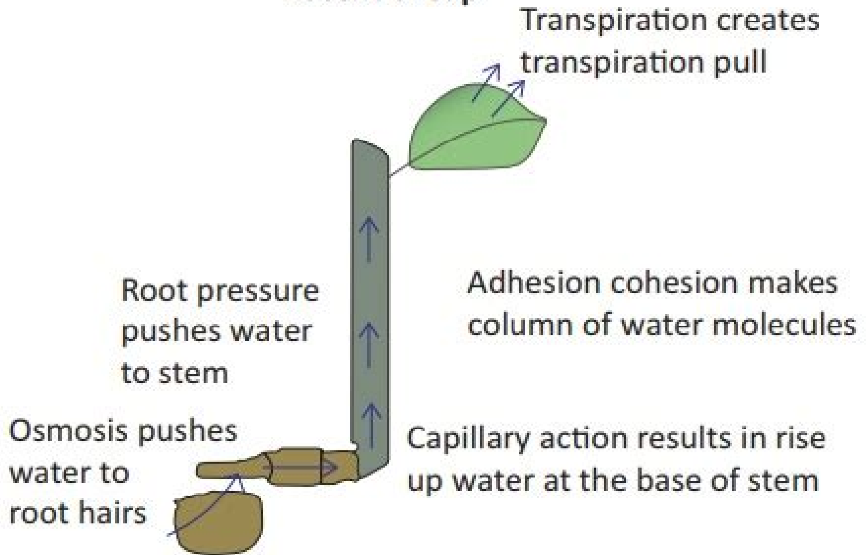
Figure 14.8 Ascent of Sap
