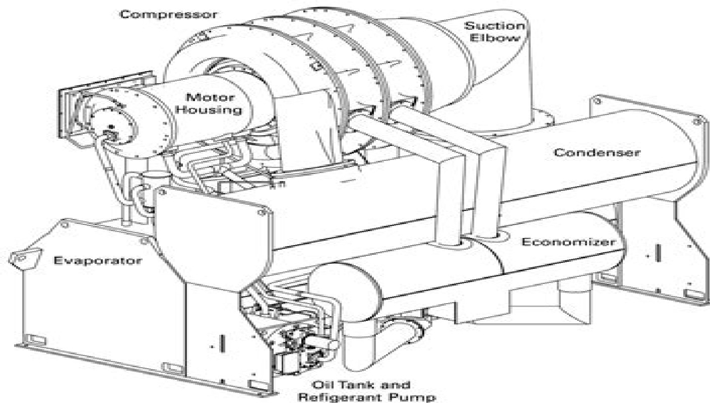
Figure 1. General CVHE and CVHG unit components - continued
