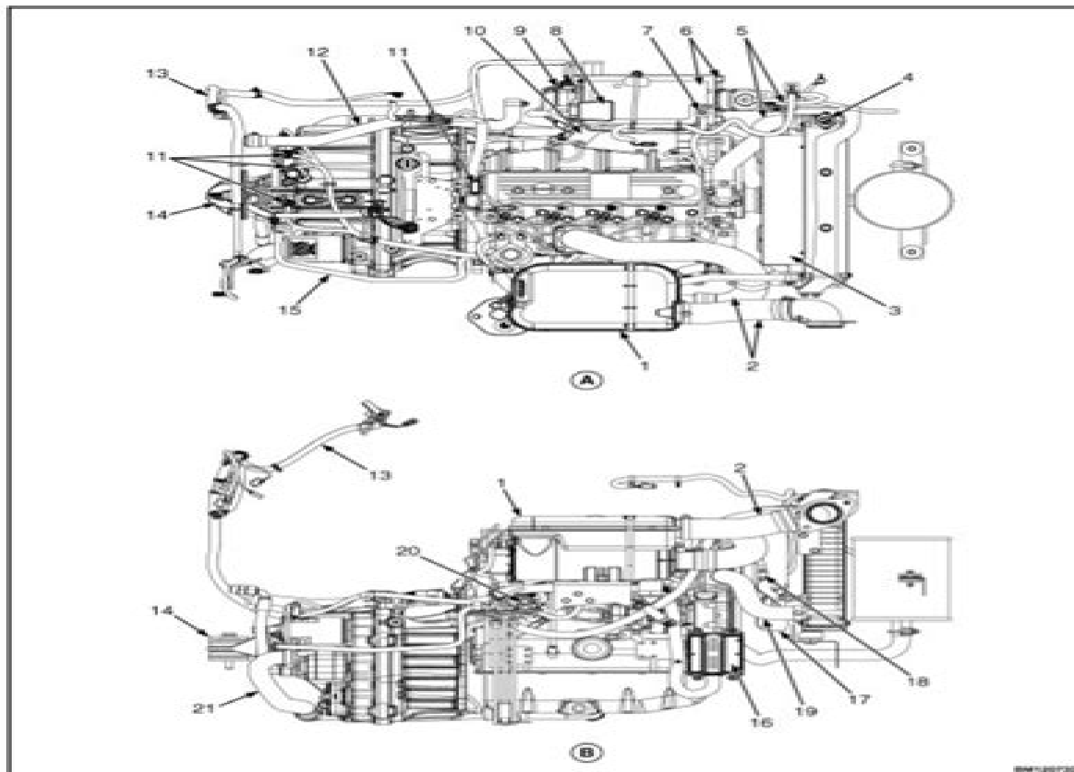
Figure 30. Yanmar 2.6L Diesel Engine and Transmission Removal
