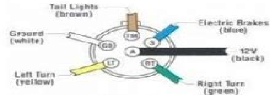
6 Way Vehicle End
