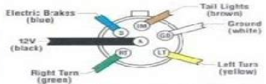
6 Way Trailer End
