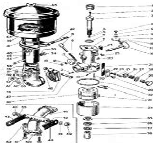
CARBURETTOR (Type V)
