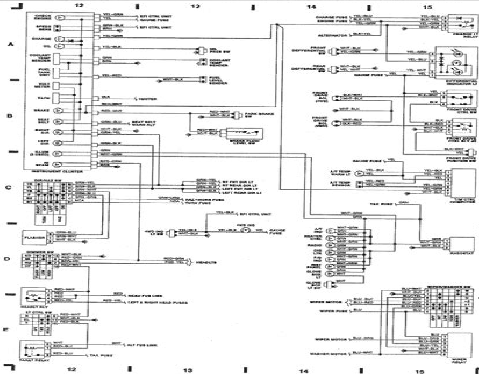
Fig. 4: Instrument Panel (Cont.) & Rear Compartment, Cluster, Hazard, Wiper/Washer 1988 Toyota Land Cruiser
