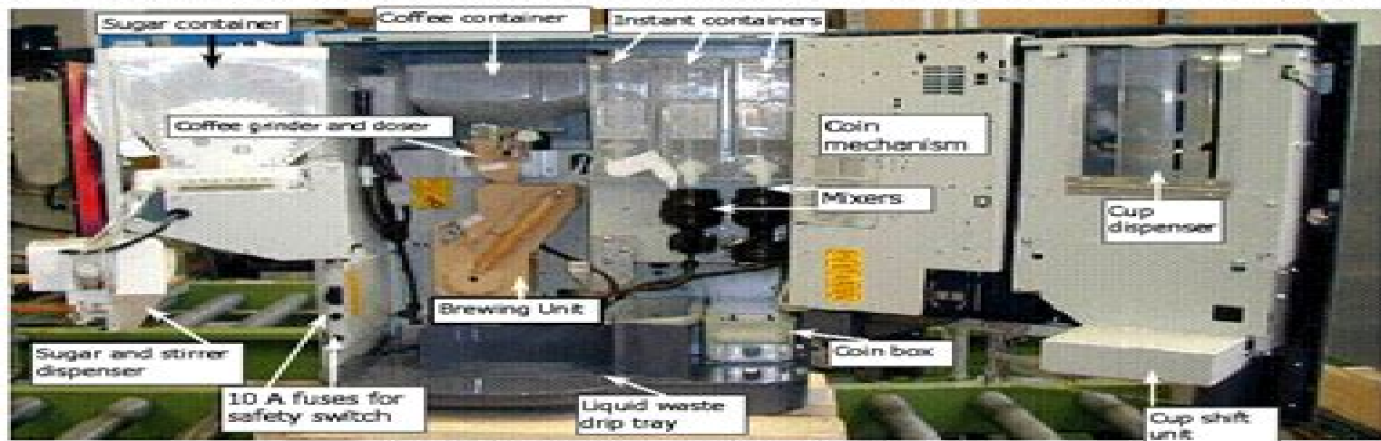
BRIO 250: VIEW WITH DOOR OPEN
