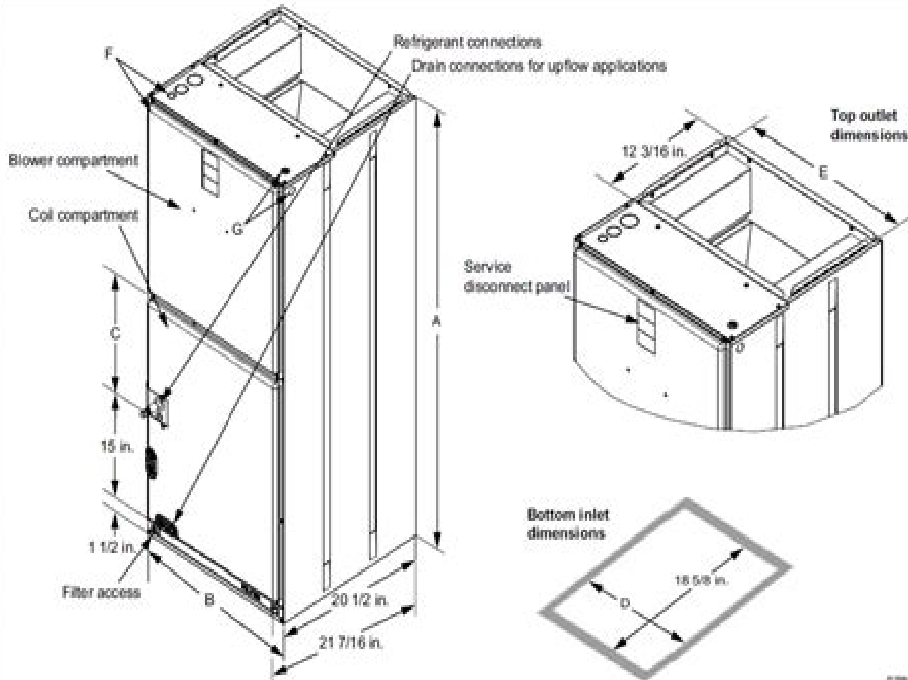
Figure 3: Dimensions and duct connection dimensions
