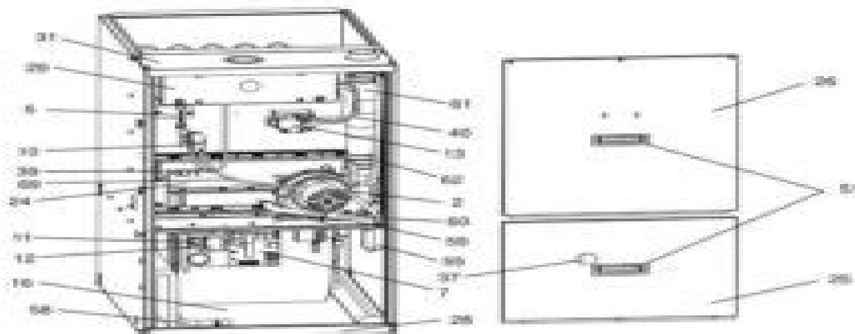
Figure 1: CONDENSING-UPFLOW NATURAL GAS FURNACES
