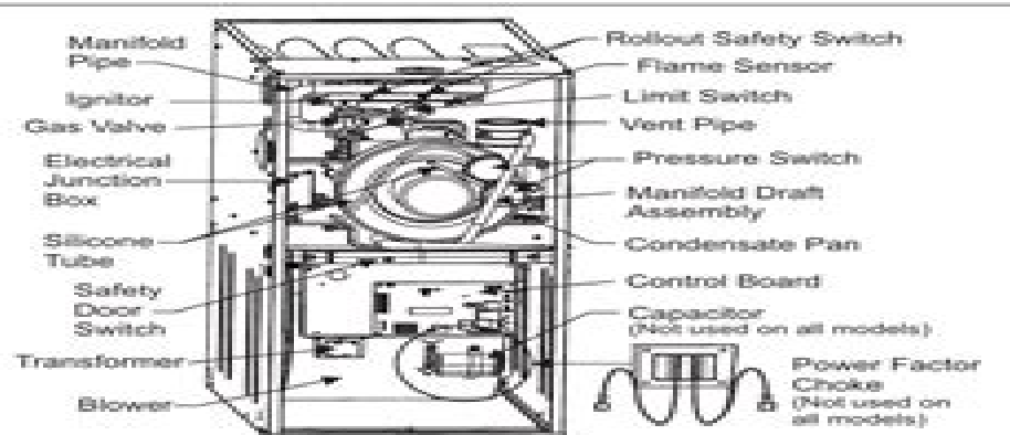
FIGURE 2: Component Location - 95% Single & 95% Two Stage Models
