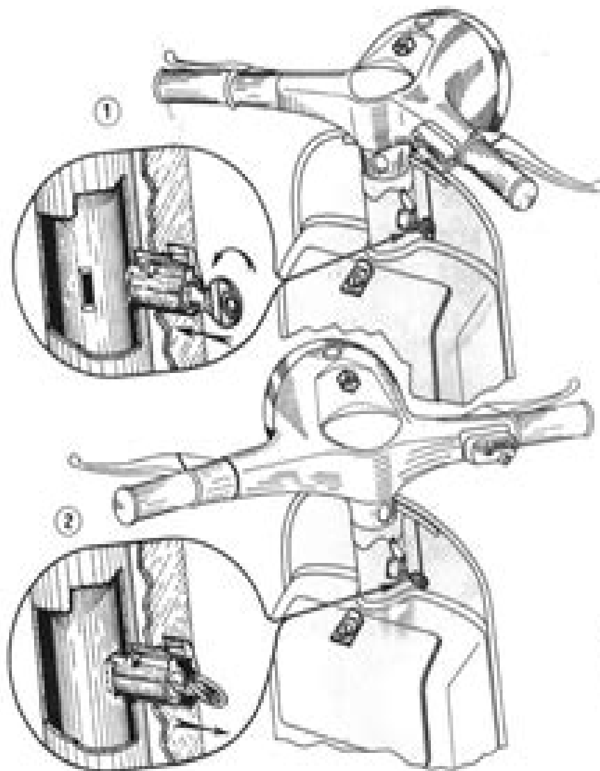
Fig. 3 - Steering lock on the steering column 1. Normal position and locking operation - 2. Locked position and unlocking operation.
