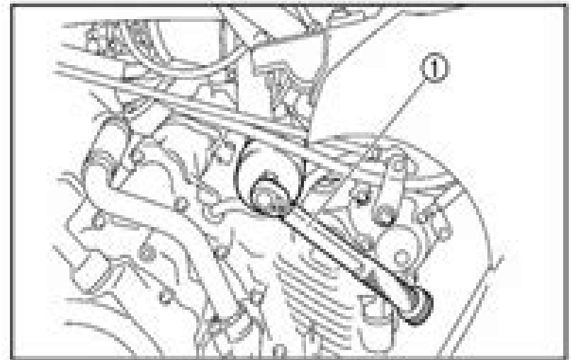
1. Torque wrench
