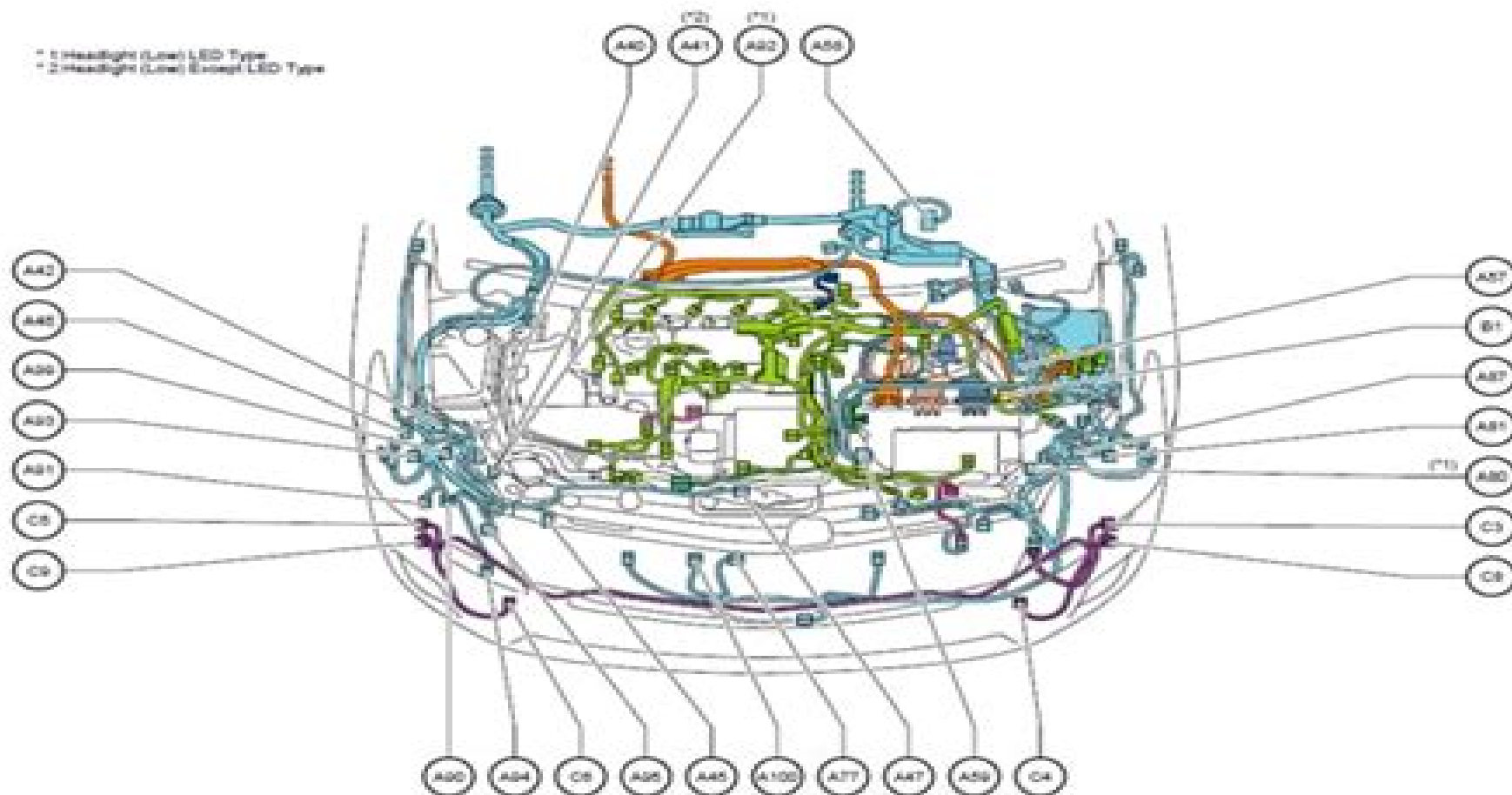
Position of Parts in Engine Compartment
