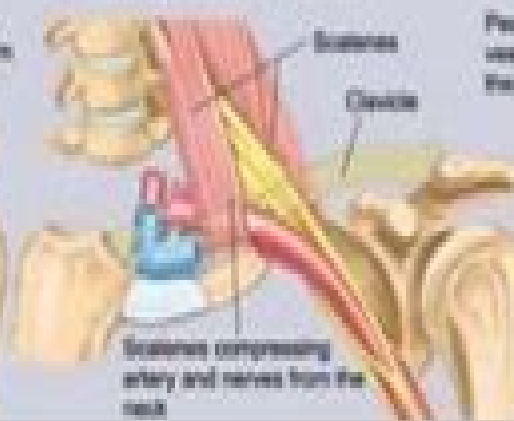
Scalene-antius syndrome
