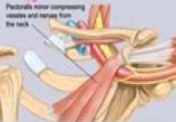
Hyperabduction syndrome
