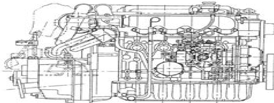
Model 4JH3-DTE(with KM4A marine gear)
