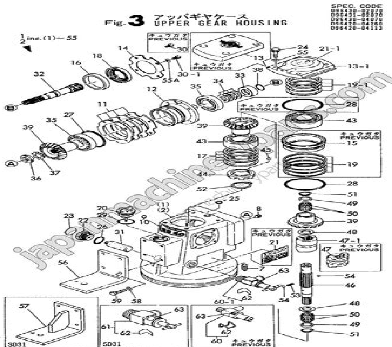
Fig.3.UPPER GEAR HOUSING
