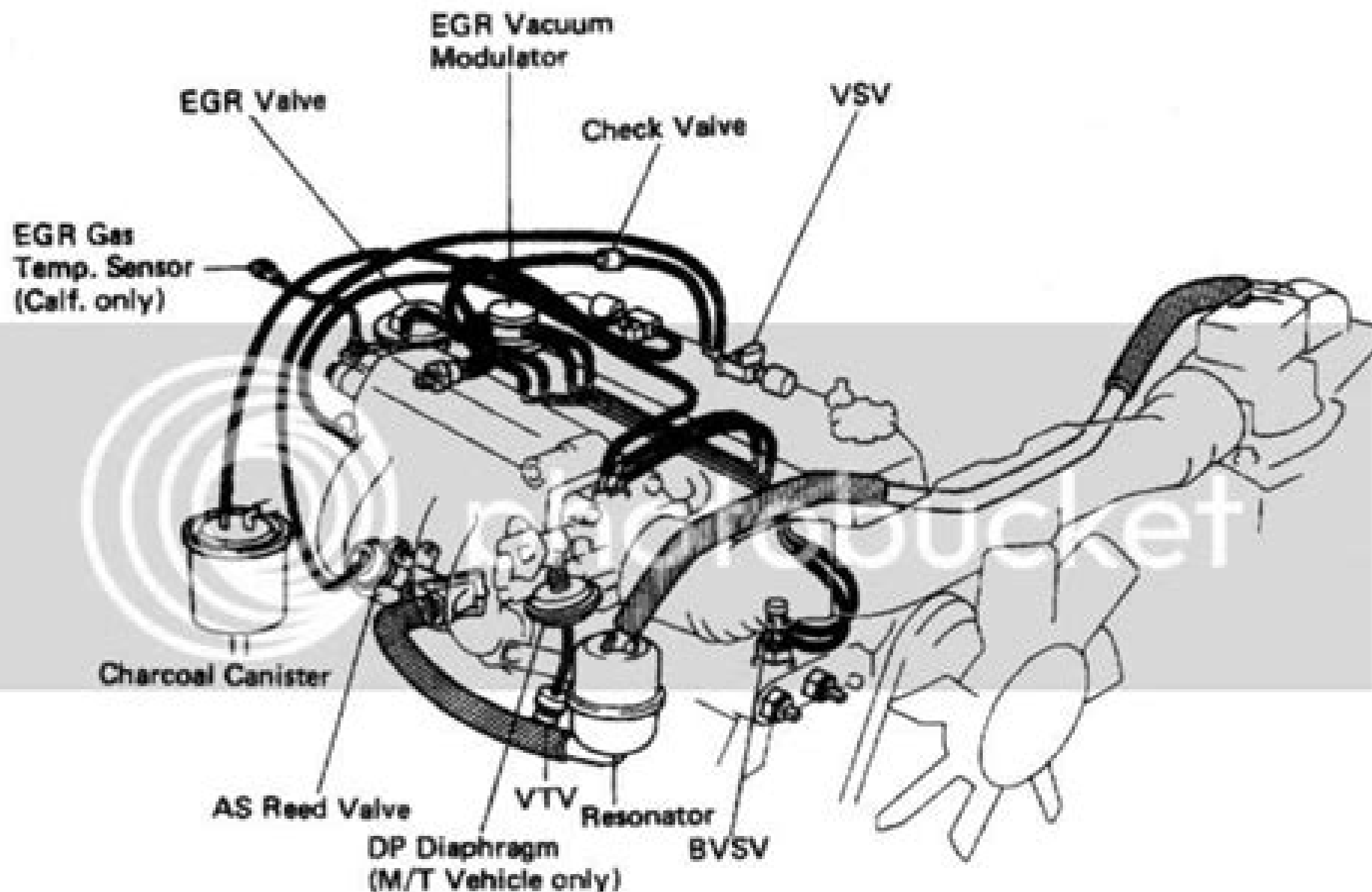
Emissions control system layout – EFI models 1988 and 1989
