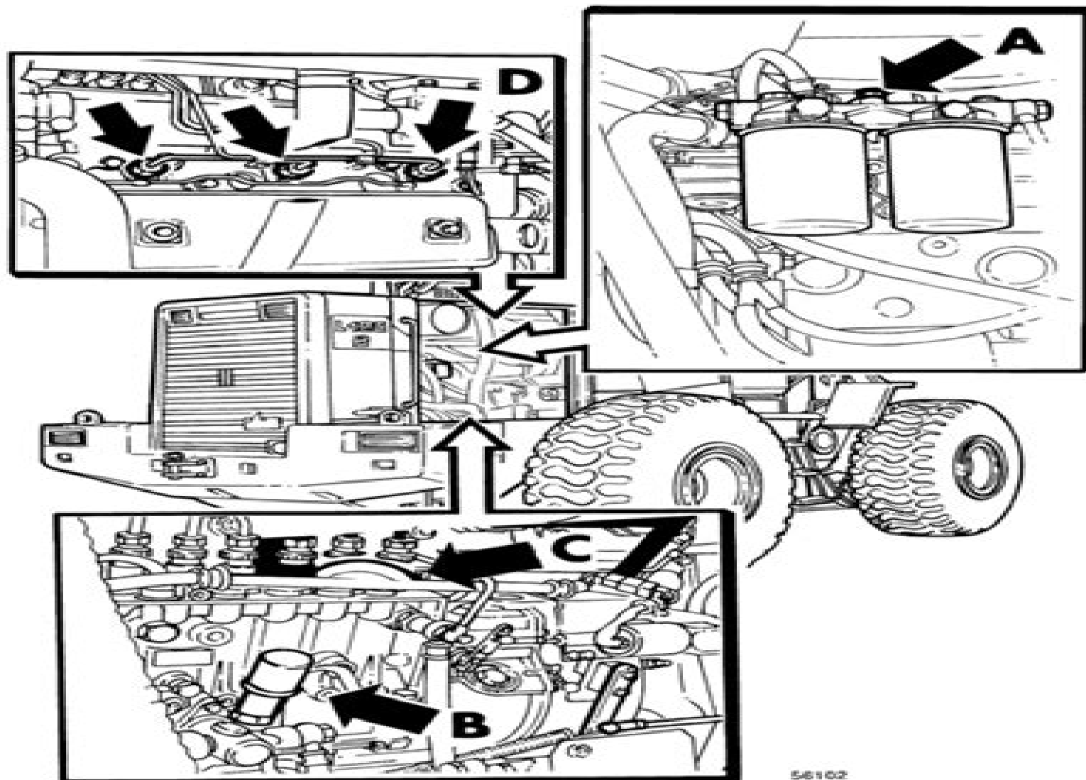
Figure 46 Fuel system, bleeding, L120B
