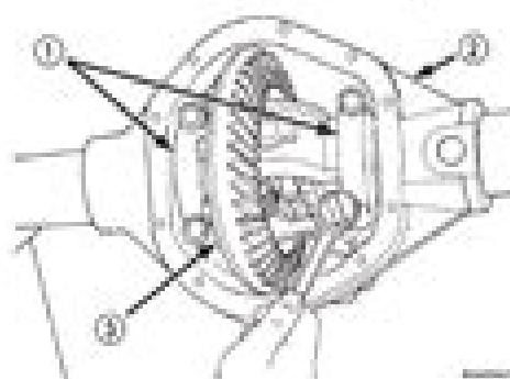
Fig. 12 Tighten Bolts Holding Bearing Cap
