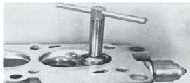
97. Clean the valve seats with a cutter. Remove carbon deposits from combustion chambers and the valves. The valve seats must not show signs of being cracked nor any other type of damage. Should this be the case, they must be replaced.
