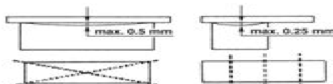
96. Clean the cylinder head and sealing surface. Use a metal ruler and feeler gauge. The warp must not exceed 0.5 mm (0.0197") lengthwise and 0.25 mm (0.0098") diagonally.
