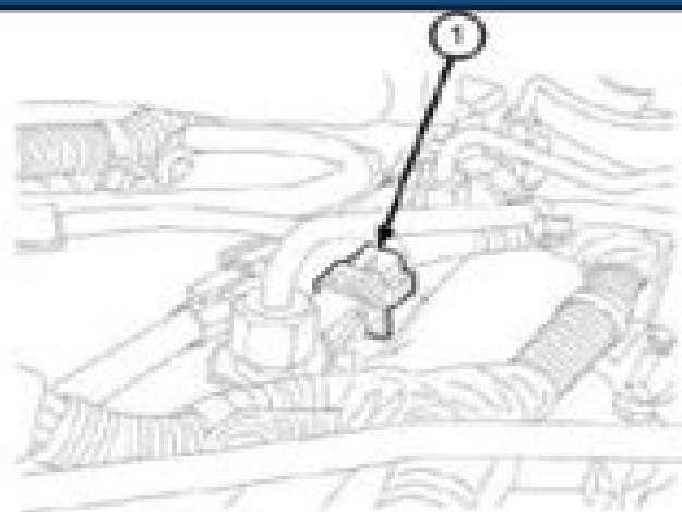
Fig. 19: Fuel Injector Connectors Courtesy of CHRYSLER LLC
