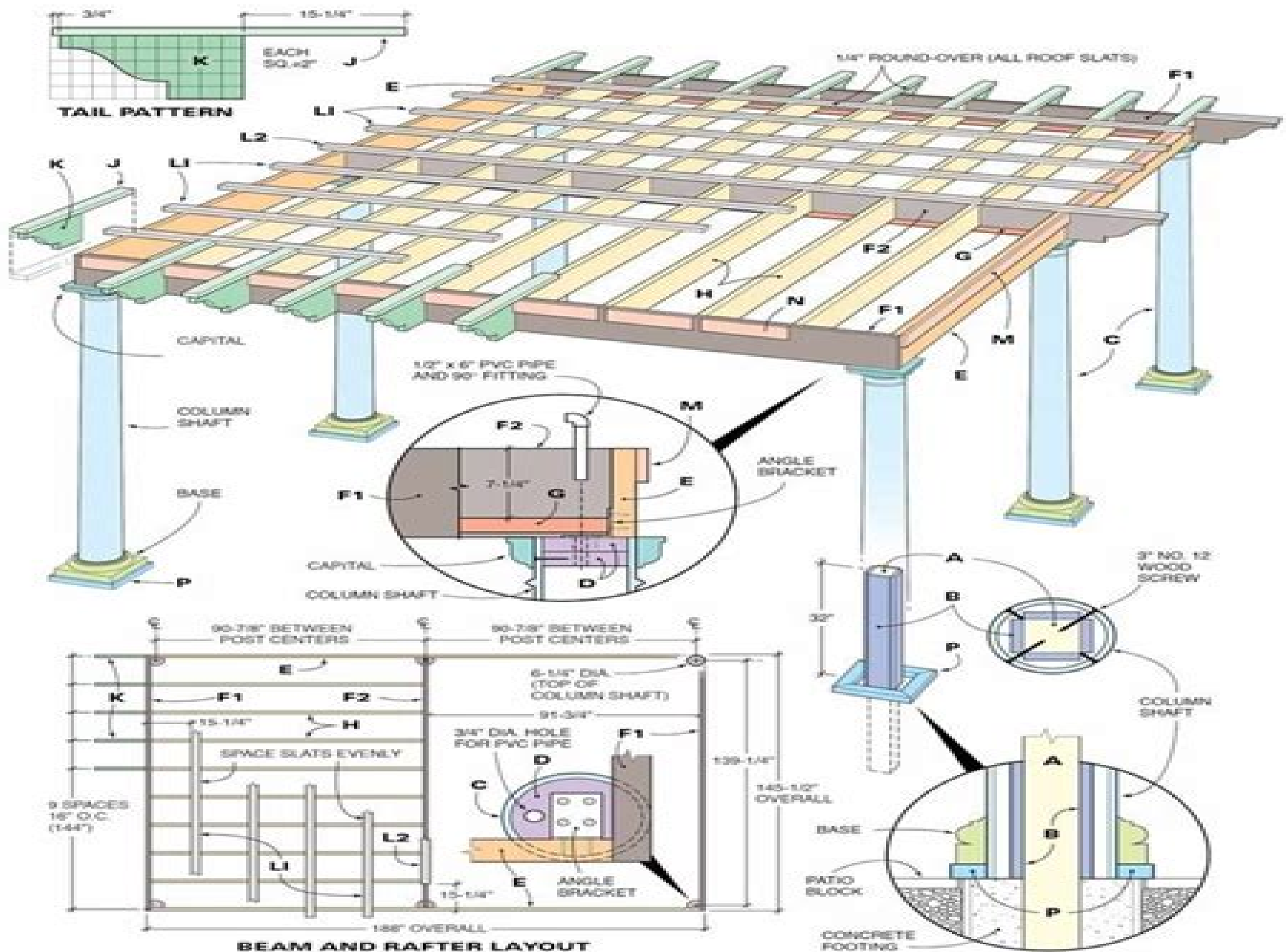
Figure A: Pergola Details
